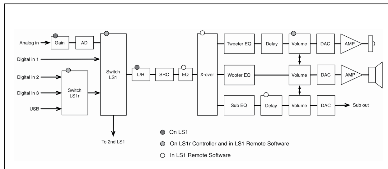
Internal flow diagram of LS1
