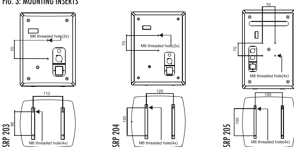
FIG. 3: MOUNTING INSERTS
