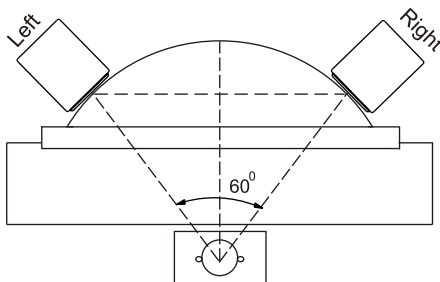
FIG. 4: STEREO SET-UP
